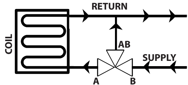
Three-Way Diverting Valve Piping Diagram (1 input, 2 Outputs)
